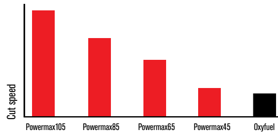
Relative cut performance on 12 mm mild steel
